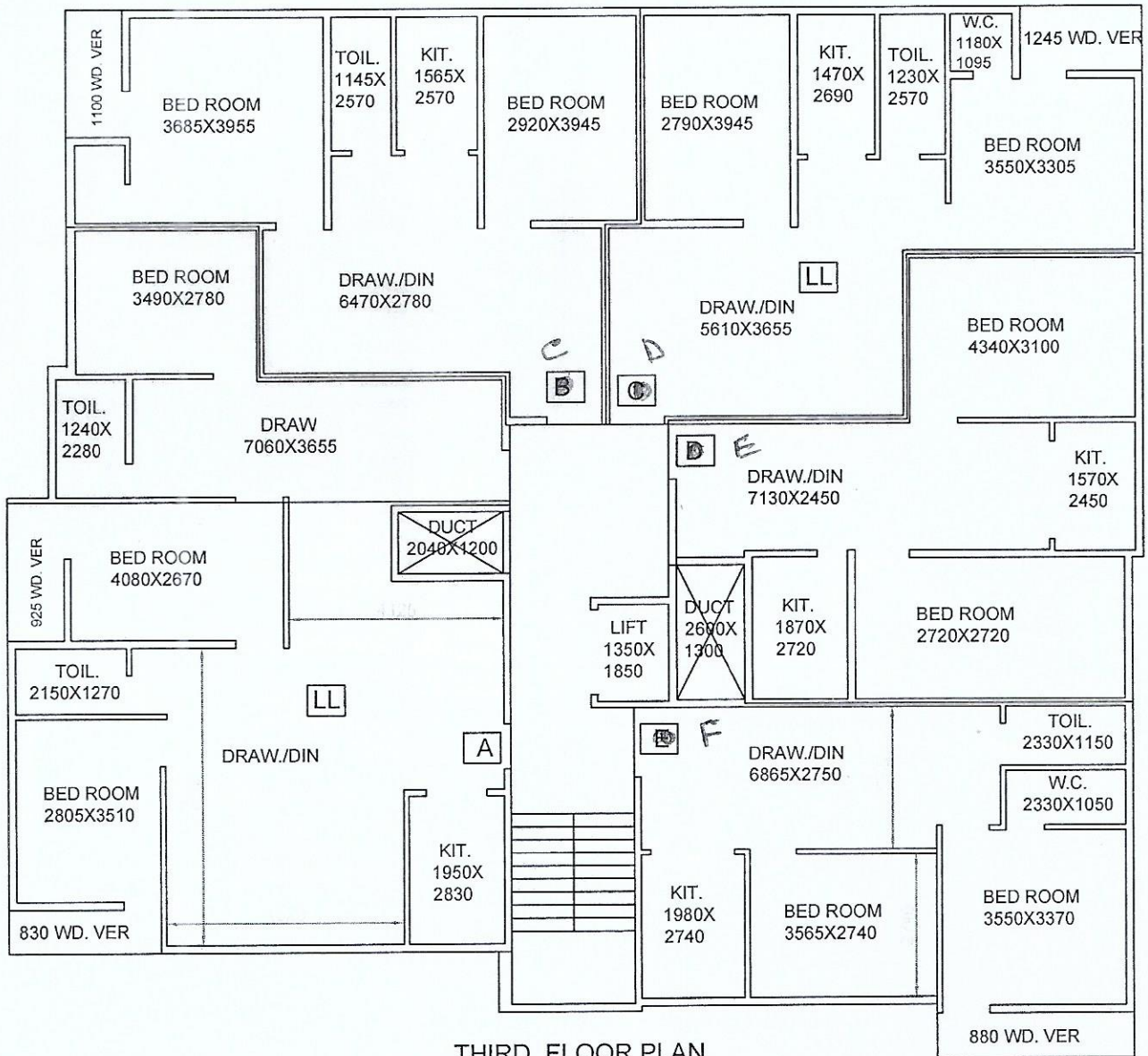
THIRD FLOOR PLAN COVERED AREA 401.90 SQM./ 4324 SFT. AREA OF STAIR, LIFT & DUCT 36.79 SQM./ 396 SFT.
